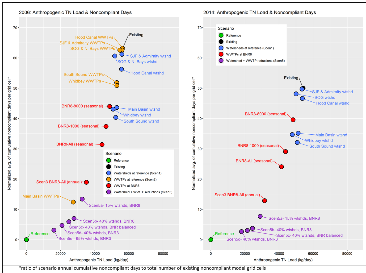
Figure 9. Comparison of normalized average predicted noncompliant days per model grid cell in WA waters of the Salish Sea resulting from all Optimization Scenarios and BNR8 Scenarios, with each scenario's associated anthropogenic total nitrogen loading in 2006 (left) and 2014 (right).
