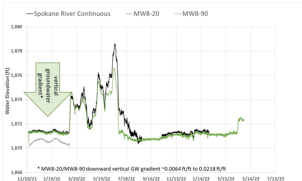
Figure 15. Graph of continuous groundwater level monitoring data for clustered wells MW8-20 and MW8-90, showing a consistent downward vertical gradient for the period late November 2021 through March 2, 2022.
