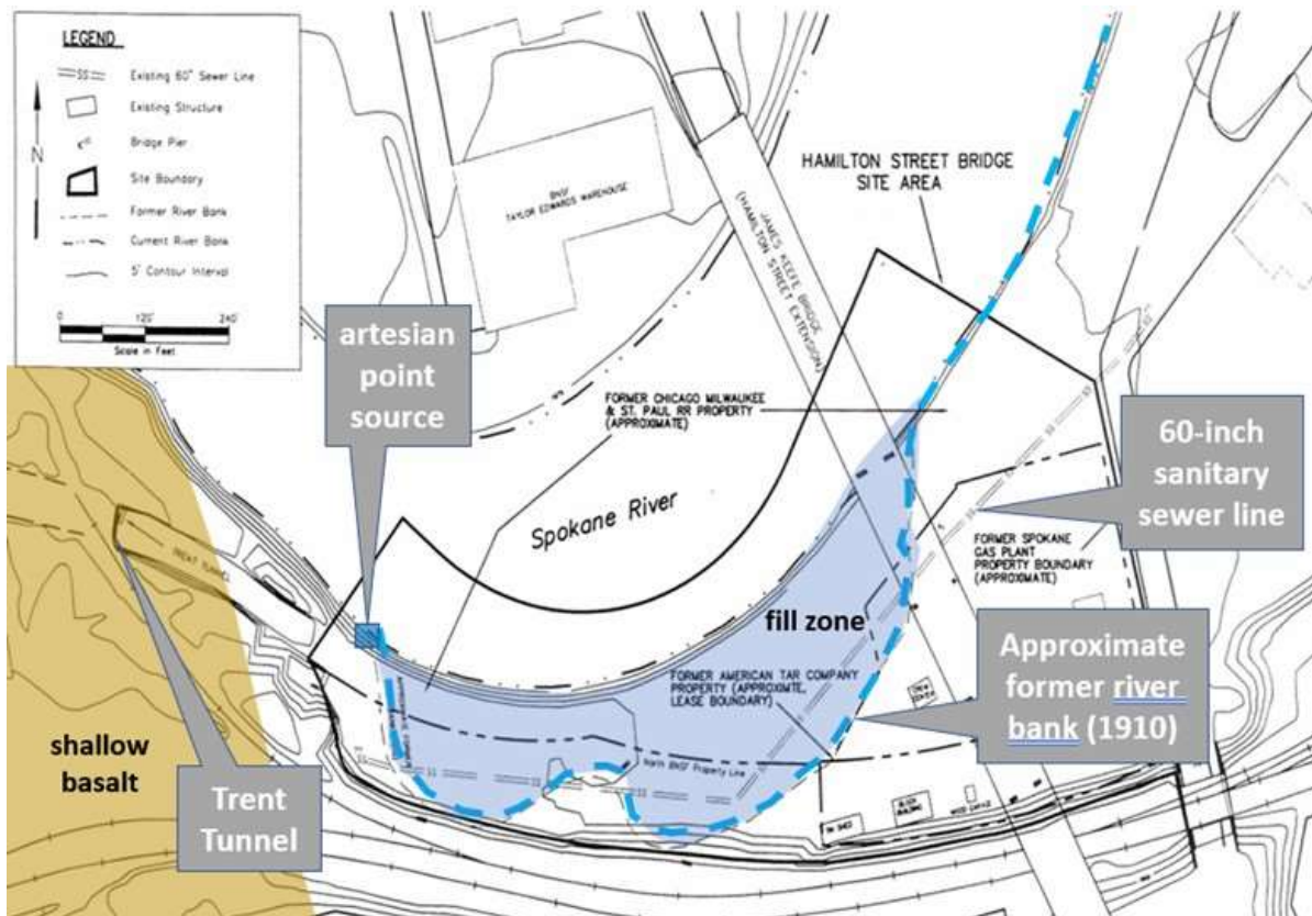
Figure 23. Location of artesian point source/well relative to shallow basalt ridge, former river bank (vintage 1910)/fill zone, 60-inch sanitary sewer line and Trent Tunnel (lower figure is modified from State of Washington Department of Ecology, July 2004).
