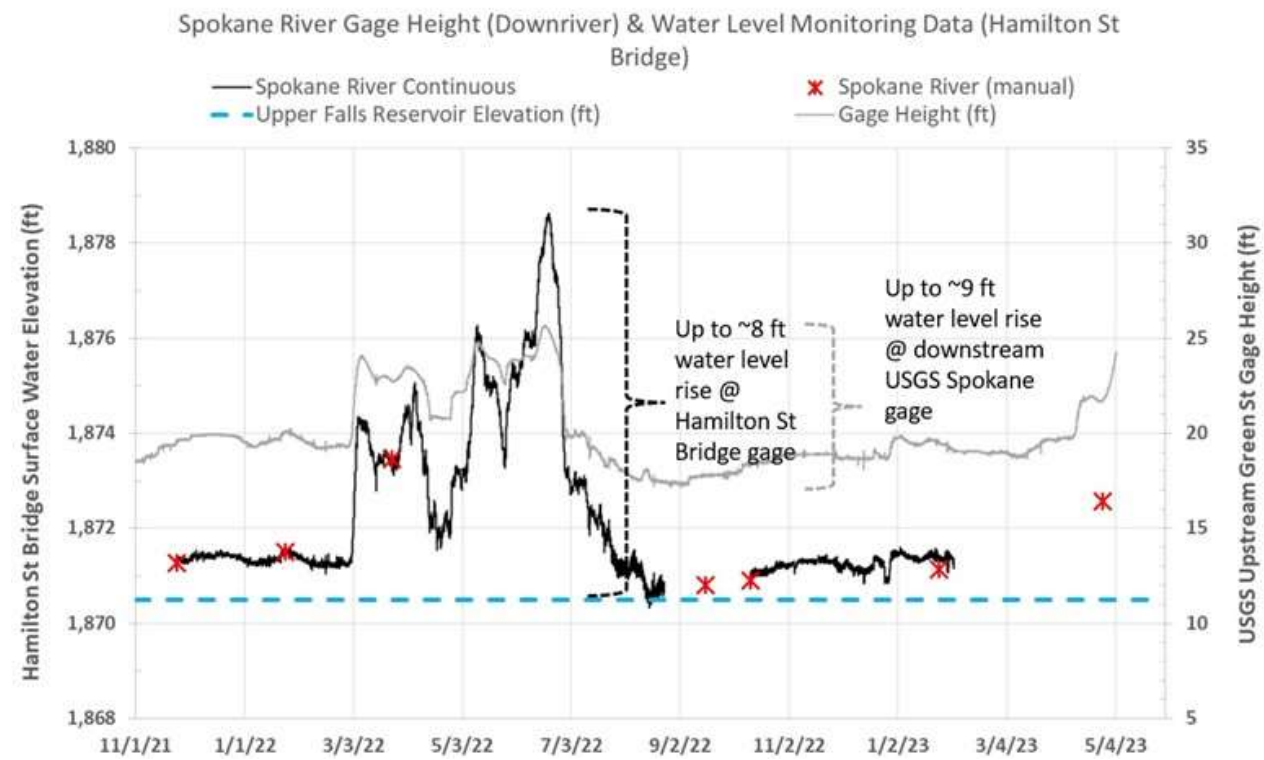
Figure 10. Continuous and manual surface water level monitoring data for the Hamilton Street Bridge study area and USGS Spokane flow and gage data.
