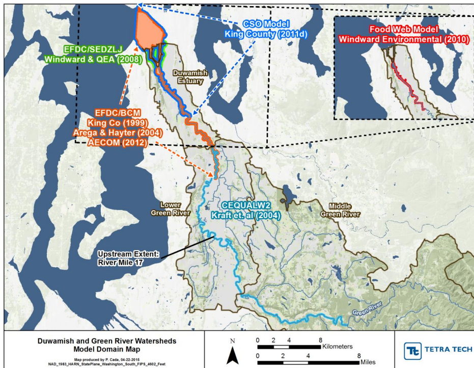
Figure 13. EFDC model domain
