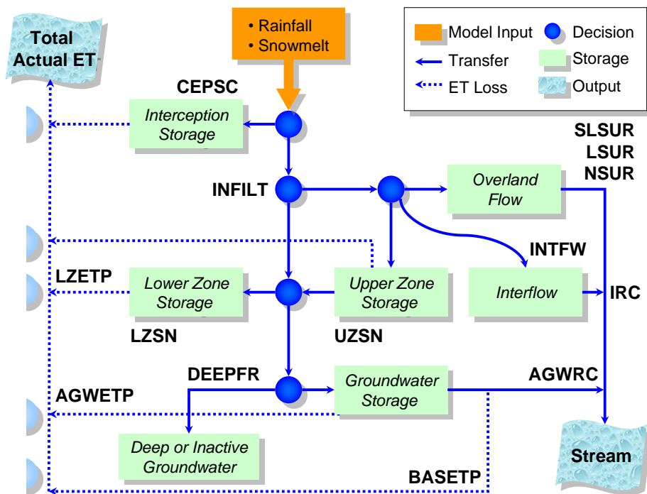
Figure 12. Hydrologic representation in the HSPF model
