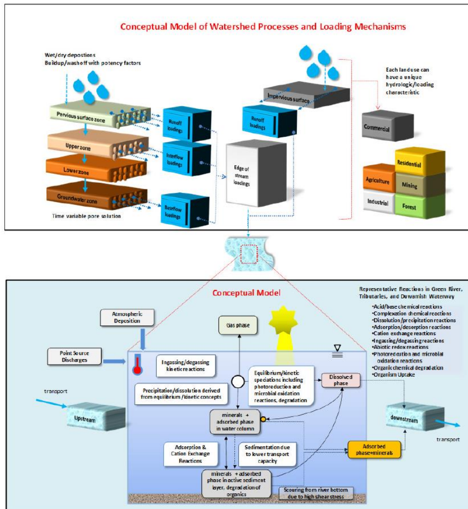
Figure 9. Watershed process and loading mechanisms
