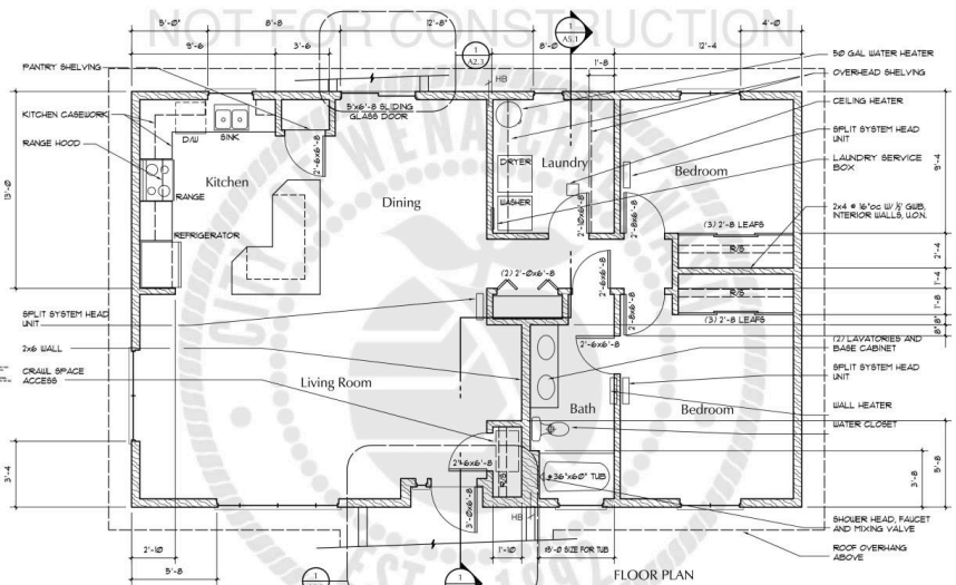
1200-1 sf 1 Story Cottage V1 City of Wenatchee/East Wenatchee Washington A0.0
