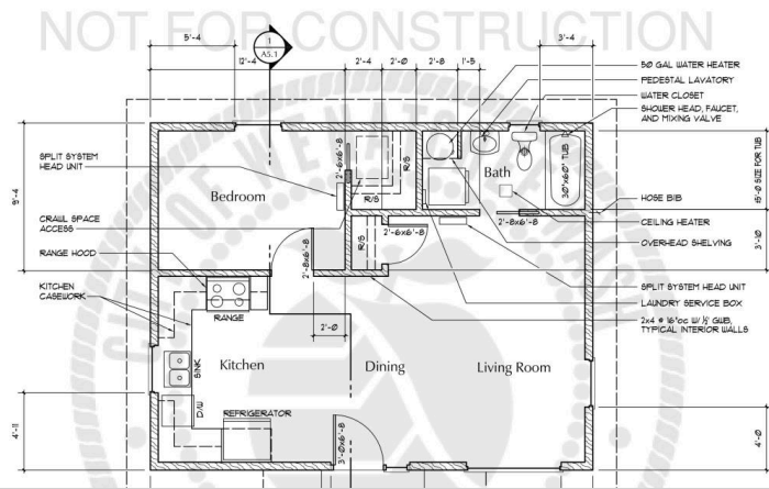
600 sf Accessory Dwelling Unit WUI1 City of Wenatchee/East Wenatchee Washington A0.0
