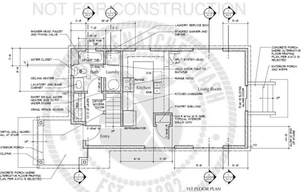
1200-2 sf 2 Story Cottage V1 City of Wenatchee/East Wenatchee Washington
