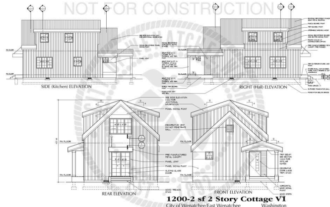
1200-2 sf 2 Story Cottage V1 City of Wenatchee/East Wenatchee Washington | A0.0
