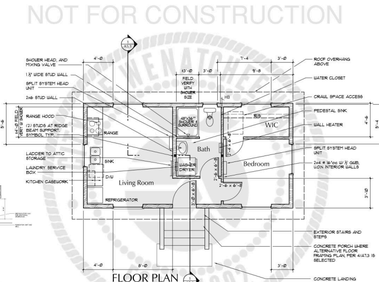
400 sf Accessory Dwelling Unit V1 City of Wenatchee/East Wenatchee Washington
