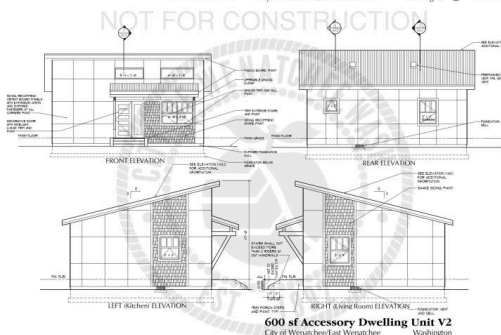
600 sf Accessory Dwelling Unit V2 City of Wenatchee/East Wenatchee Washington A0.0
