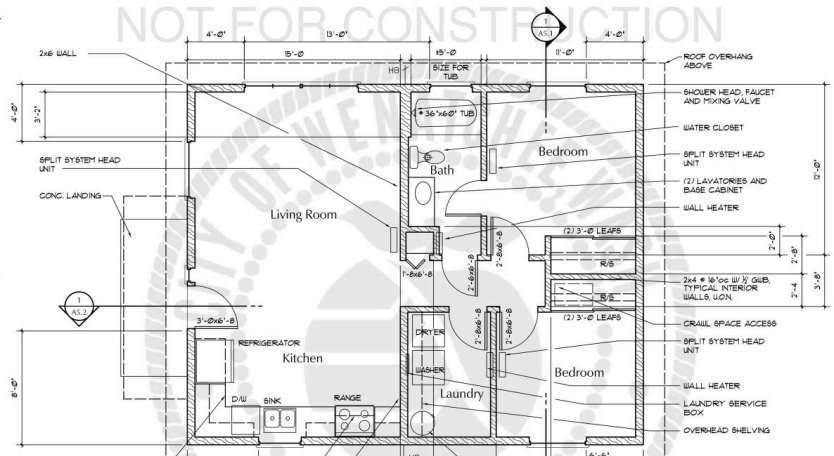
800 sf Accessory Dwelling Unit WUI 1 City of Wenatchee/East Wenatchee Washington A0.0
