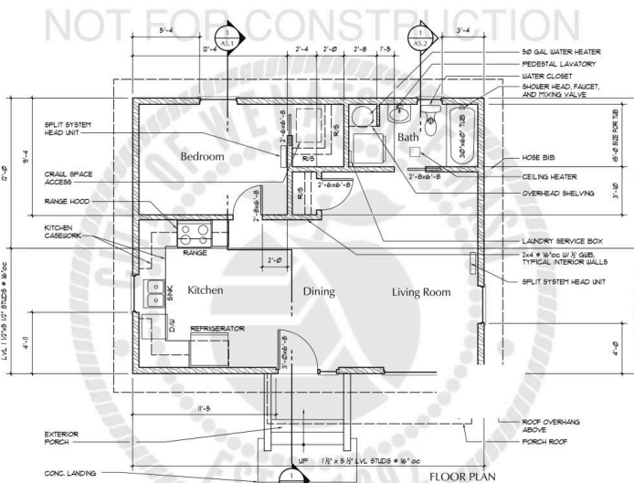
600 sf Accessory Dwelling Unit V2 City of Wenatchee/East Wenatchee Washington
