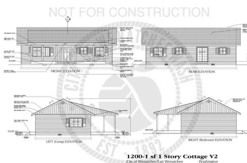
1200-1 sf 1 Story Cottage V2 City of Wenatchee/East Wenatchee Washington A0.0
