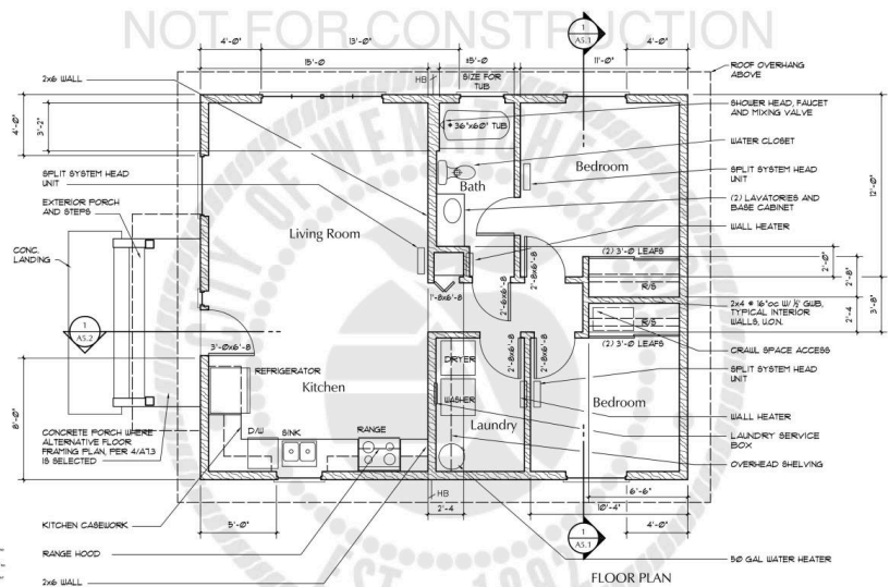
800 sf Accessory Dwelling Unit V1 City of Wenatchee/East Wenatchee Washington
