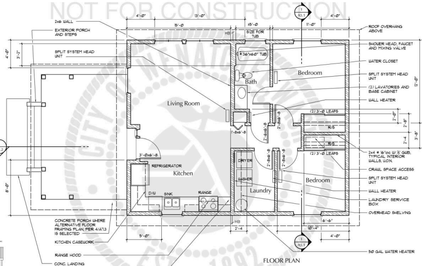
800 sf Accessory Dwelling Unit V2 City of Wenatchee/East Wenatchee Washington
