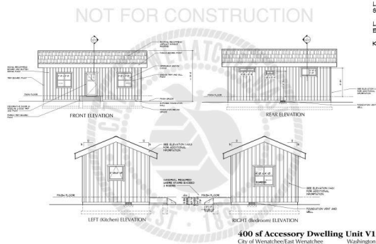
400 sf Accessory Dwelling Unit V1 City of Wenatchee/East Wenatchee Washington
