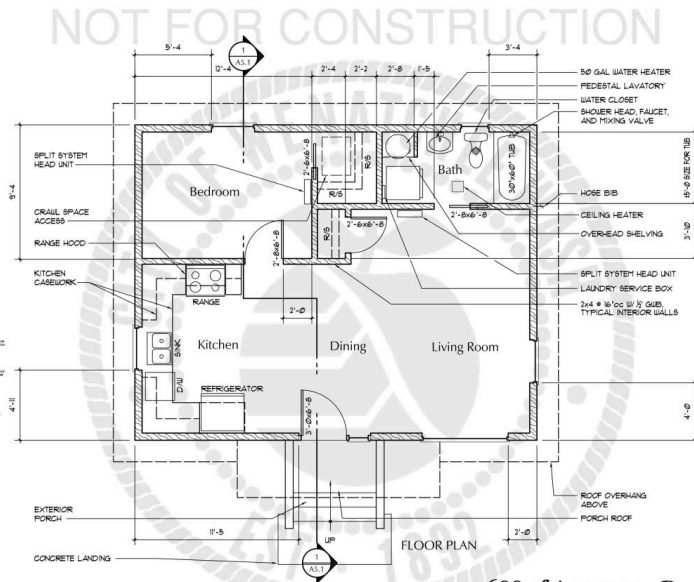
600 sf Accessory Dwelling Unit V1 City of Wenatchee/East Wenatchee Washington
